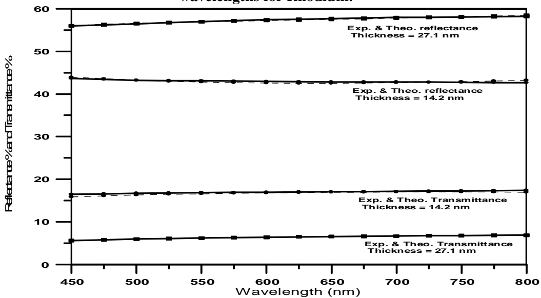
Figure (4) Experimental and Theoretical reflectance and transmittance versus wavelength for Rhodium.
