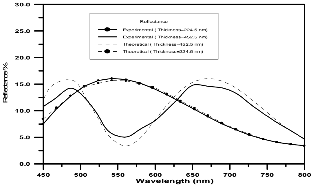
Figure (2): Experimental and Theoretical reflectance versus wavelength for Scandium Oxide.
