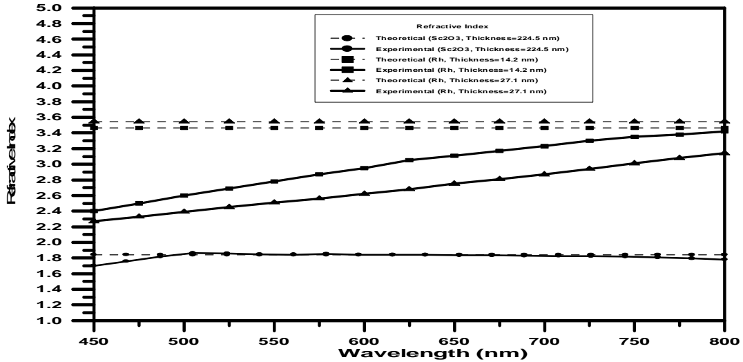
Figure (1) Experimental and theoretical refractive index versus wavelength for Scandium Oxide and Rhodium.
