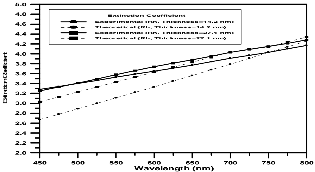
Figure (3) Experimental and theoretical extinction coefficients versus wavelengths for Rhodium.
