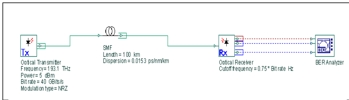
Fig. (5): The experiment setup of optical fiber communication system with using DFF.
