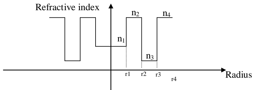
Fig. (2): Index profiles four layer fiber structures
