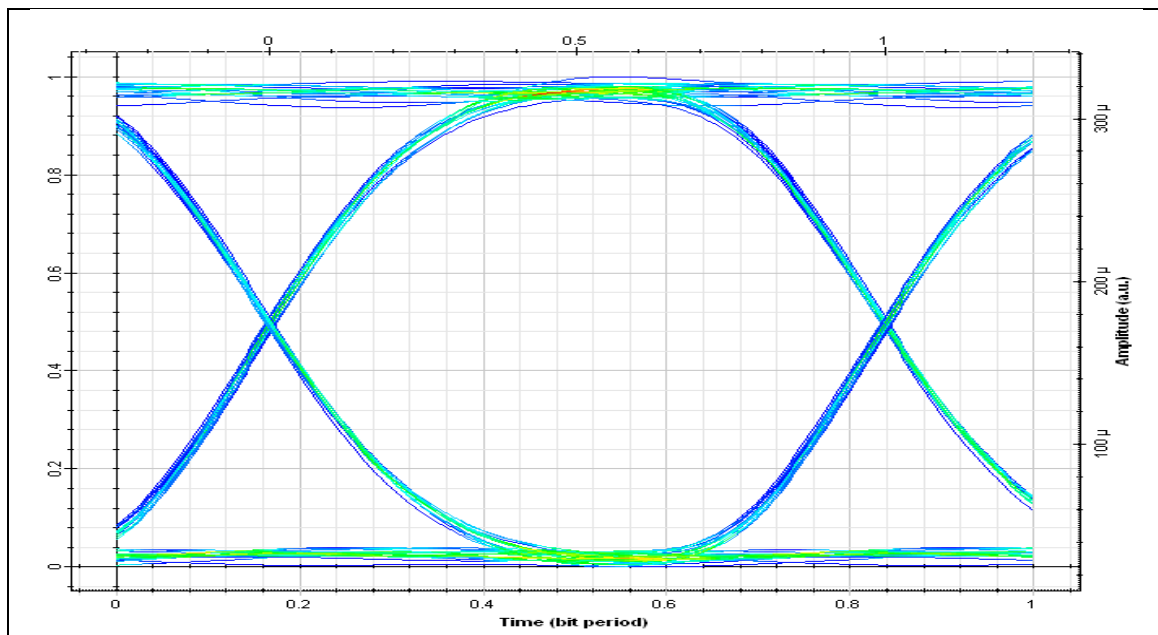
Fig. (6-a): Illustrate the eye diagram of NRZ formats transmit over optical transmission system with using DFF of length 50km.
