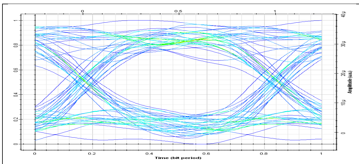
Fig. (6-b): Illustrate the eye diagram of NRZ formats transmit over optical transmission system with using DFF of length 100km.
