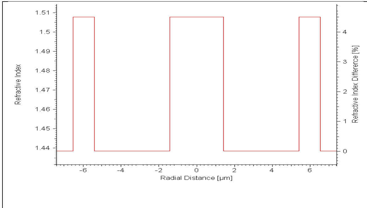
Fig. (3): Index profiles of proposed four layer fiber structure
