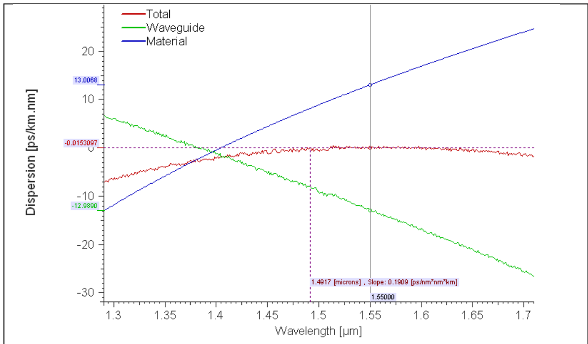
Fig. (4): The relation between the total dispersion versus wavelength.
