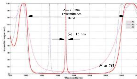
Figure (3) transmittance as function of wavelength for three cases ( F_3 Represent shifting of 110 nm with structure G(HL)^6 0.6L(HL)^6 LG , F_2 which represent the structure G(HL)^6 L(HL)^6 LG that is the phase shift version of the dielectric mirror structure, F_1 which represent Dielectric mirror of G(HL)^6 |G structure).
