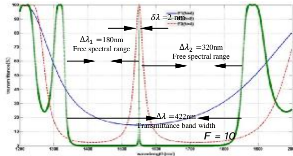
Figure (8) transmittance as function of wavelength for three cases (F2 Represent N=88 with structure G(\text{HL})^6 \text{L}(\text{HL})^6 \text{LG} , F3 represent N=4 which represent the structure G(\text{HL})^4 \text{L}(\text{HL})^4 \text{LG} that is the phase shift version of the dielectric mirror structure with N=4 , F1 represent Dielectric mirror of G|(\text{HL})^4 |G structure with N_1=4 ).
