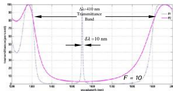
Figure (2) transmittance as function of wavelength for two cases ( F_2 which represent Dielectric mirror of G|(HL)^6|G structure, F_1 represent the structure G(HL)^6L(HL)^6 LG which is the Phase shift version of the dielectric mirror structure).
