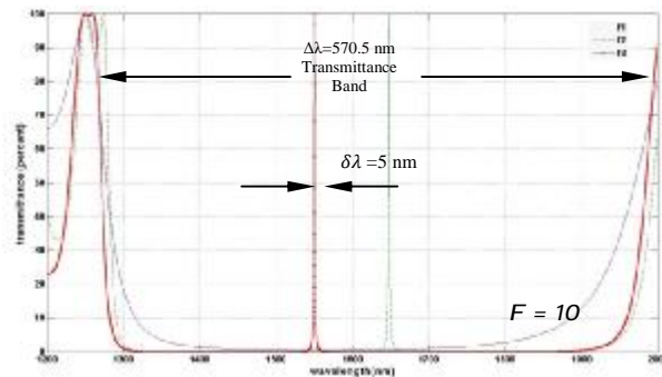
Figure(6) transmittance as function of wavelength for three cases ( F_3 Represent transmission filter with single FBR of structure G(\text{HL})^6 L(\text{HL})^6 \text{LG} , F_2 represent the of transmission filter with single FBR with 1.3 thickness of the sandwiched layer with structure of G(\text{HL})^6 1.3 L(\text{HL})^6 \text{LG} , F_1 represent Dielectric mirror of G|(\text{HL})^6 |G structure).
