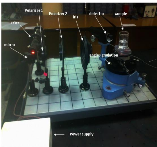
Figure (2): The setup of Nano-Particles
